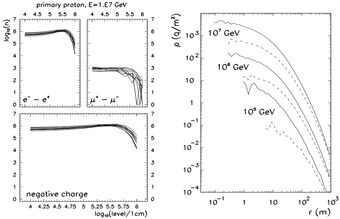
Fig. 1. Left: Excess of negative charge for primary proton 10^7 GeV versus observation level. Right: Lateral distribution of negative charge excess at 600 m a.s.l. for proton (solid lines) and iron (broken lines) initiated showers.
