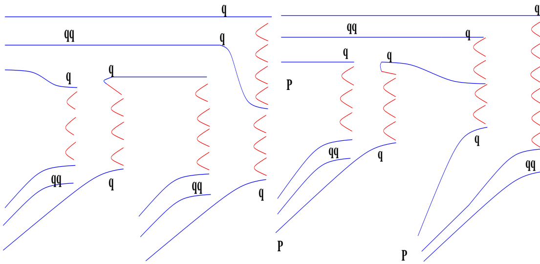
Fig. 4. Feynmann diagram of diquark breaking.
