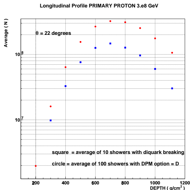
Fig. 5. Simulation with DPM model with option D (100 showers), and diquark breaking (10 showers).
